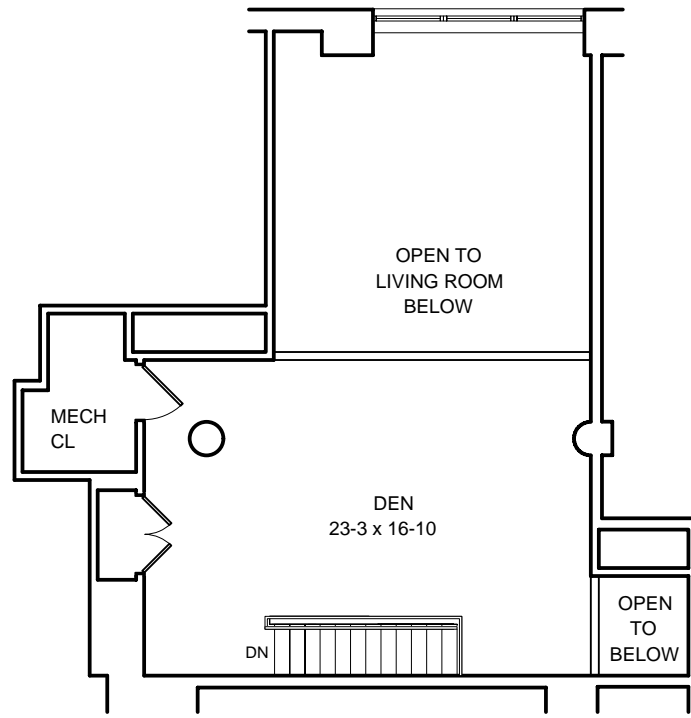
MEZZANINE LEVEL
