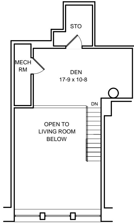
MEZZANINE LEVEL
