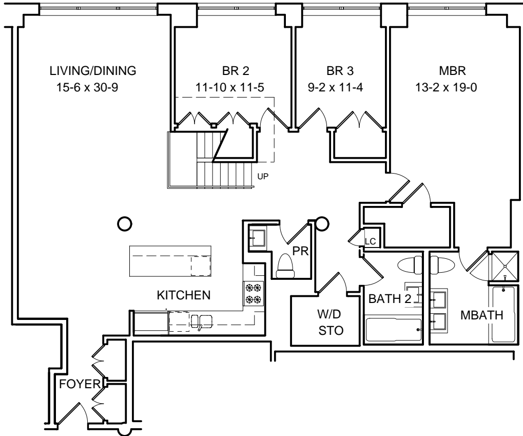
11TH FLOOR LEVEL
